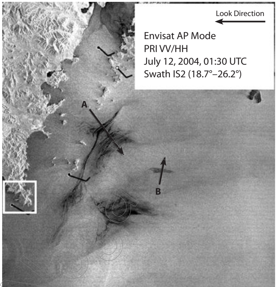
Figure 6. Envisat Advanced SAR image (ASAR; VV polarization, 100 km × 100 km) acquired during the field experiments in Vityaz Bay, Sea of Japan (see the white square on the left). Normalized radar cross section transects were calculated along lines A and B (see Figure 7). The four wind arrows indicate a northwest wind direction at the time of SAR acquisition. Image © ESA, 2004
