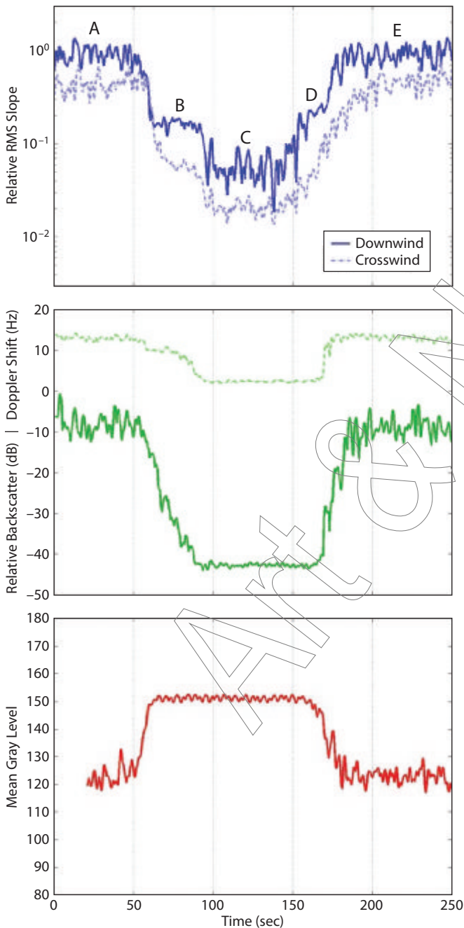
Figure 2. (upper panel) Time series of downwind and crosswind wave slope (dark and light blue curve, respectively). (middle panel) Time series of radar Doppler shifts and radar backscatter (upper and lower curve, respectively). (lower panel) Time series of mean image gray levels. Data were acquired while a small (60 seconds) palmitic acid methyl ester (PME) slick was drifting by. Wind speed was 3 \text{ m s}^{-1} .
