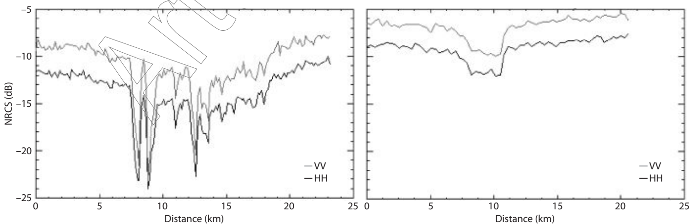
Figure 7. Normalized radar cross section (NCRS) calculated along lines A and B indicated in the Figure 6 SAR image. The upper, gray curves denote vertical (VV) polarization. The lower, black curves denote horizontal (HH) polarization.
