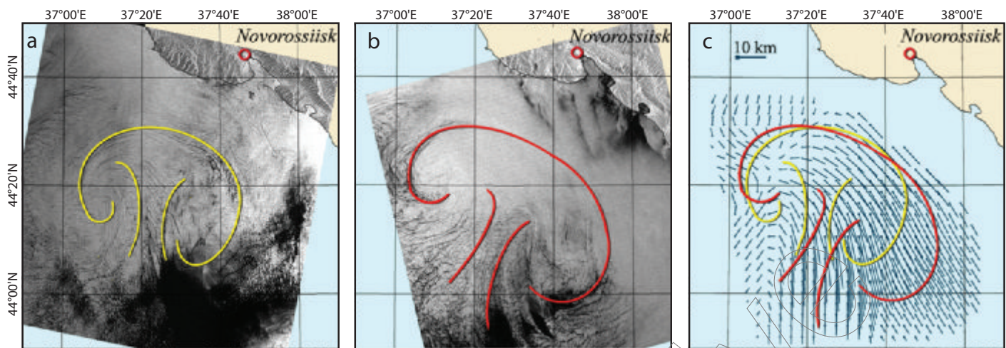
Figure 11. (a) Envisat ASAR image obtained June 19, 2006, at 07:52 GMT showing a nascent dipole eddy. Dimensions are about 66 km x 62 km. © ESA, 2006 (b) Envisat ASAR image of a 92 km x 78 km dipole eddy obtained June 19, 2006, at 19:10 GMT © ESA, 2006. (c) Reconstruction of the local velocity field from analysis of images a and b.
